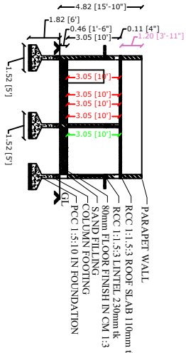
SECTION ON A-A
