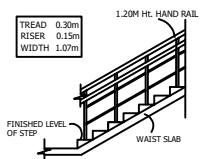
STAIRCASE DETAILS
