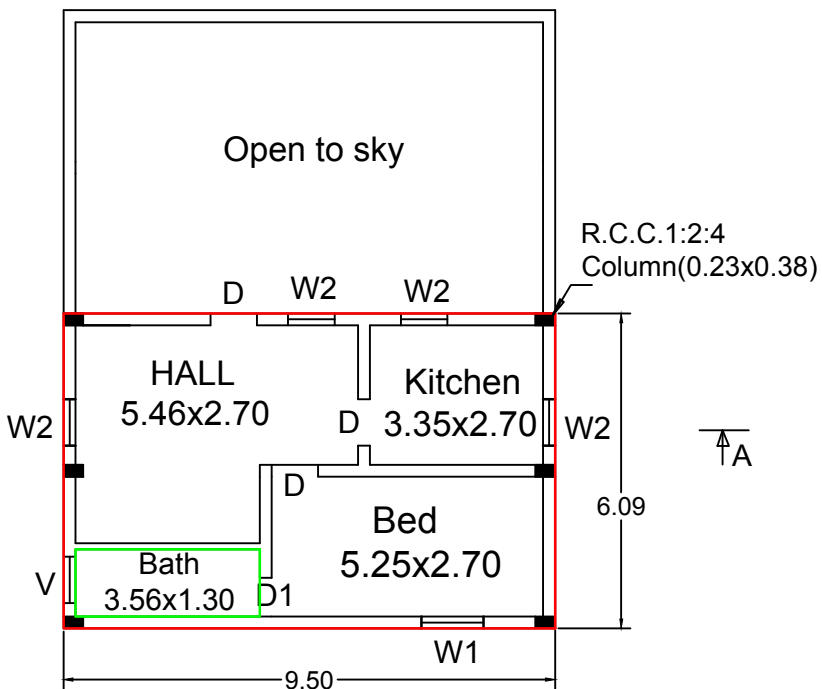
PLAN - First Floor (House)
