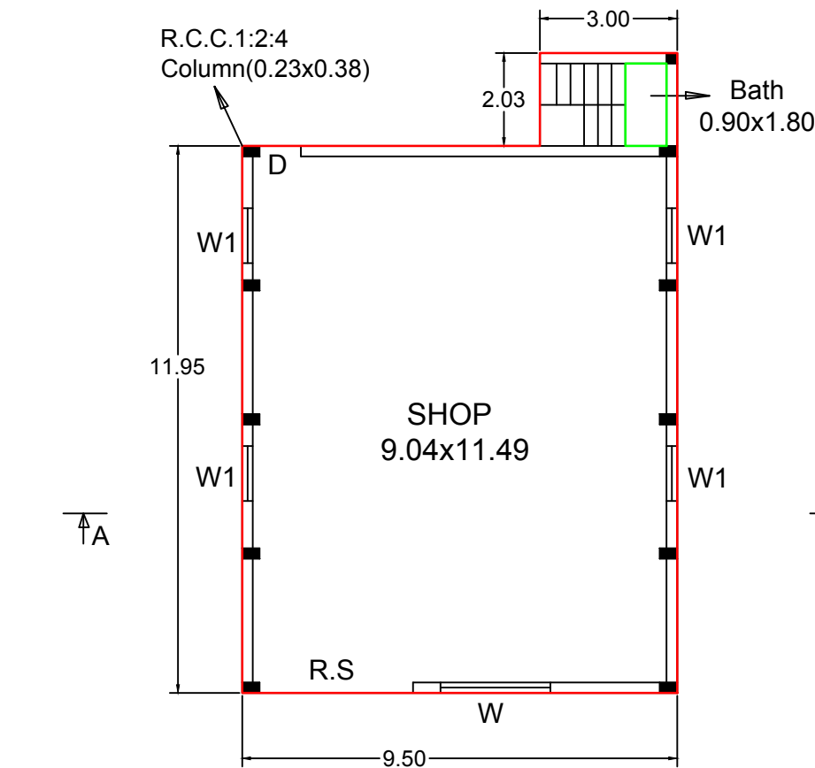
PLAN - Ground Floor(Shop)
