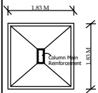
Plan of Footing
