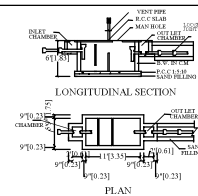
SEPTIC TANK:-
