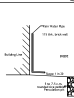
PERCOLATION PIT :
