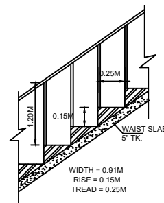
STAIRCASE DETAIL
