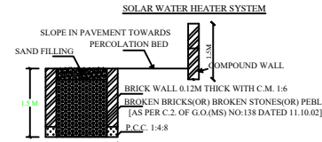
SECTION OF RAIN WATER PERCOLATION BED
