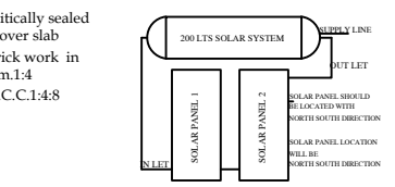
SOLAR WATER HEATER SYSTEM
