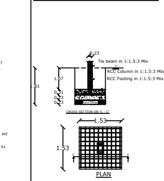
COLUMN FOUNDATION DETAILS:-
