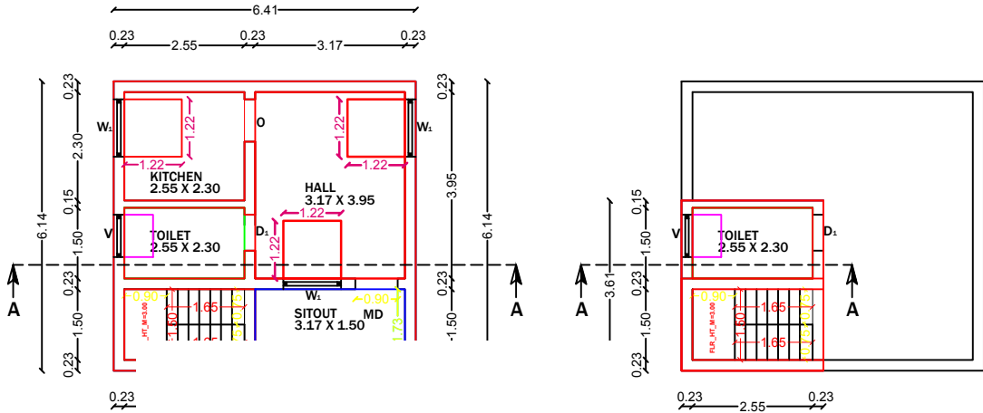
FIRST FLOOR
