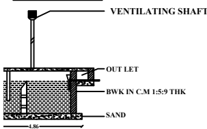
SEPTIC TANK
