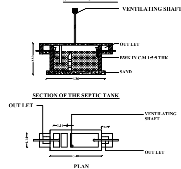
SEPTIC TANK
