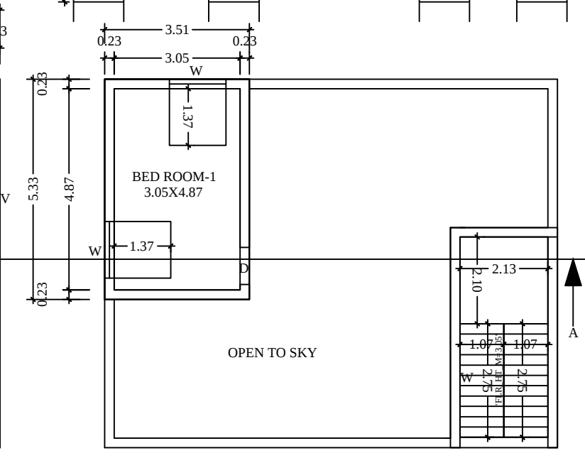
PLAN FOR FIRST FLOOR
