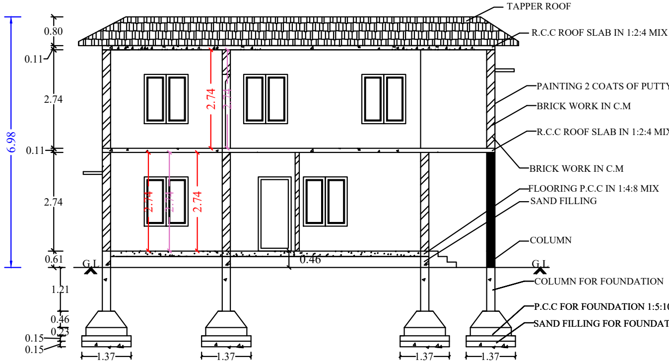
SECTION ON-AA
