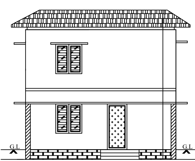
FRONT ELEVATION
