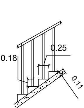
STAIRCASE DETAILS:-
