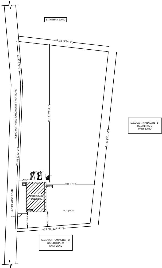
TOPO PLAN:- (SCALE 1:1000)
