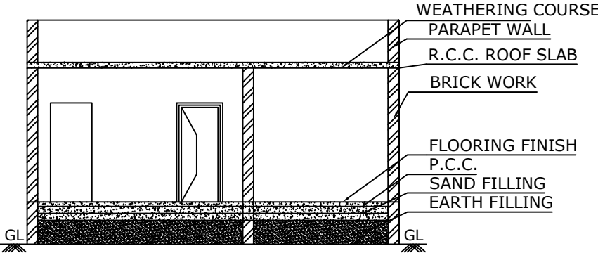
SECTION ON XX
