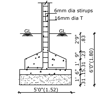
COLUMN FOUNDATION DETAIL
