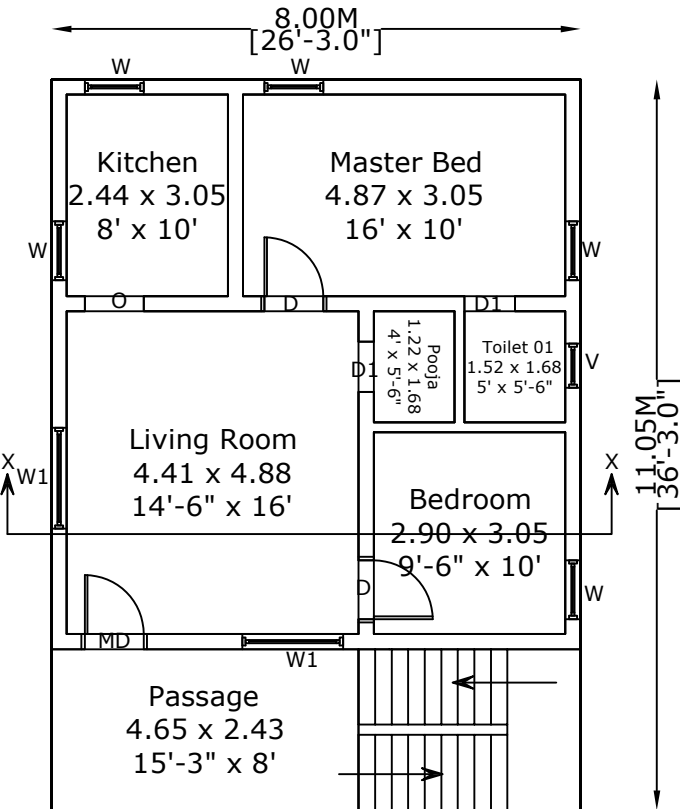
SITE CUM PRO.GROUND FLOOR
