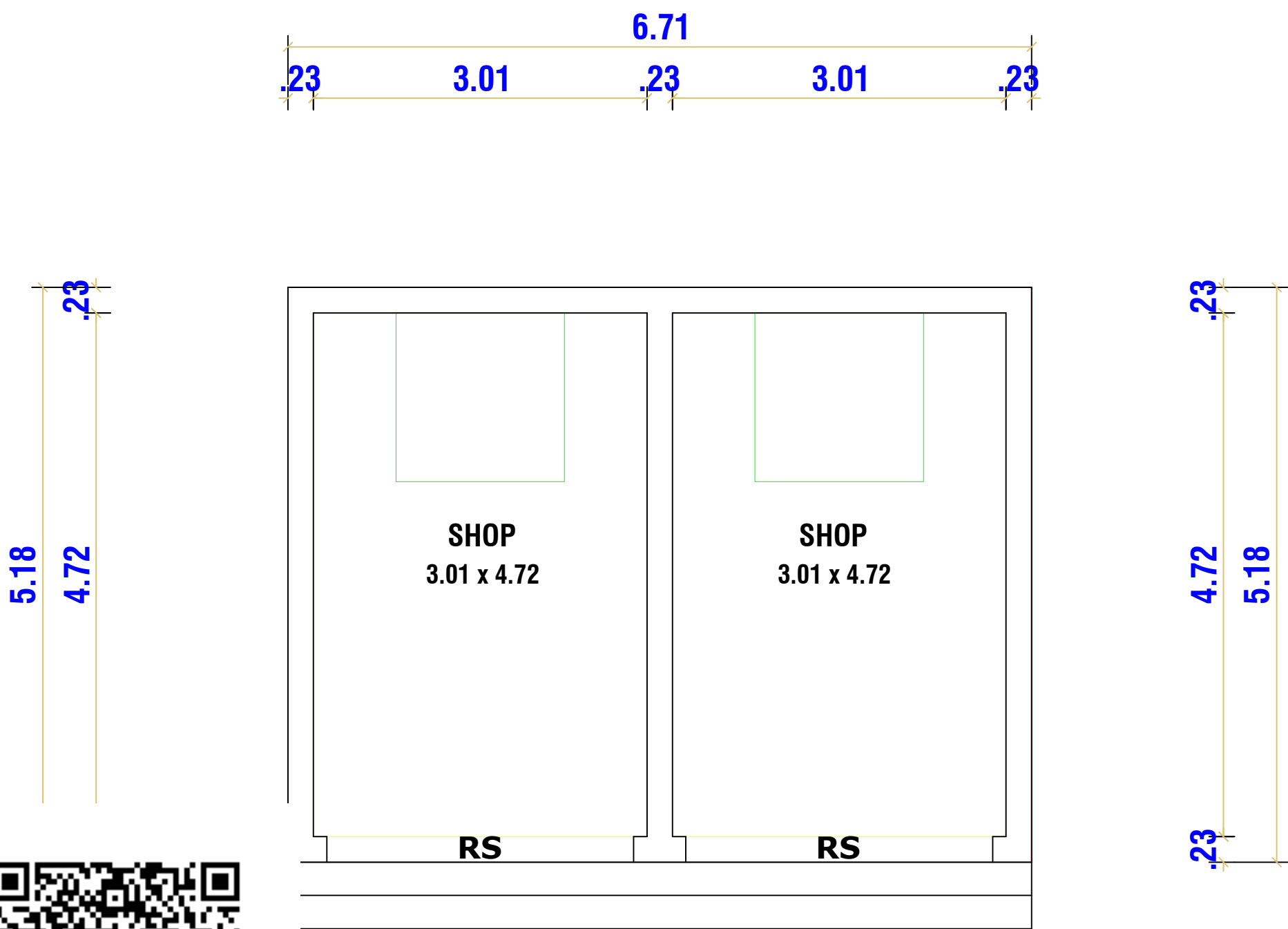
PLAN
