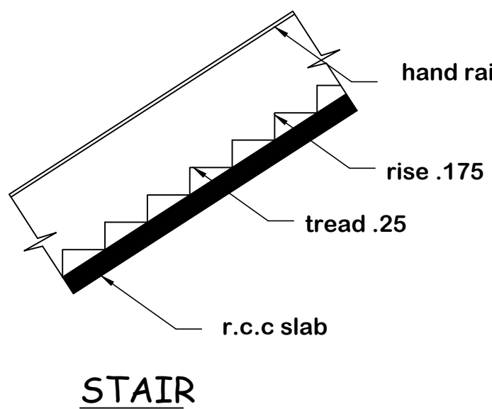
STAIR
