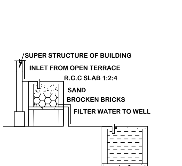
RAINWATER HARVESTING
