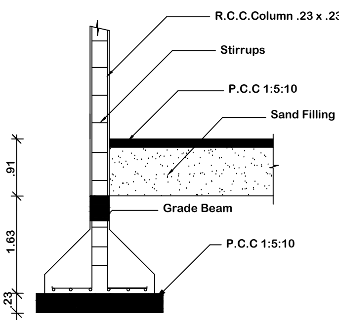
COLUMN DETAIL
