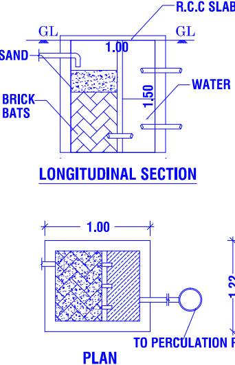
RAIN WATER HARVESTING TUB
