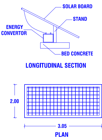
SOLAR PANEL
