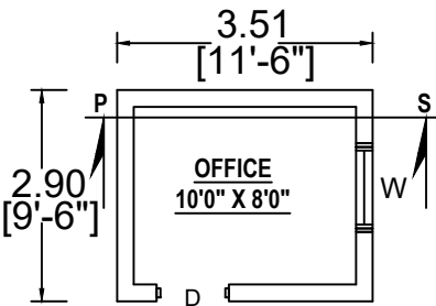
PLAN (R.C.C. ROOF)
