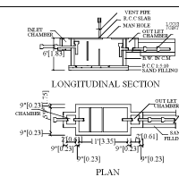
SEPTIC TANK:-
