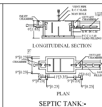
SEPTIC TANK:-
