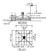
FOUNDATION DETAILS
