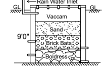
RAIN WATER HARVESTING TANK
