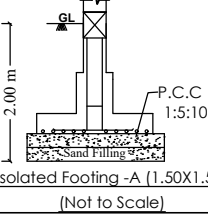
FOUNDATION DETAIL - A
