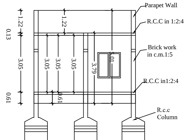
CROSS SECTION-AA
