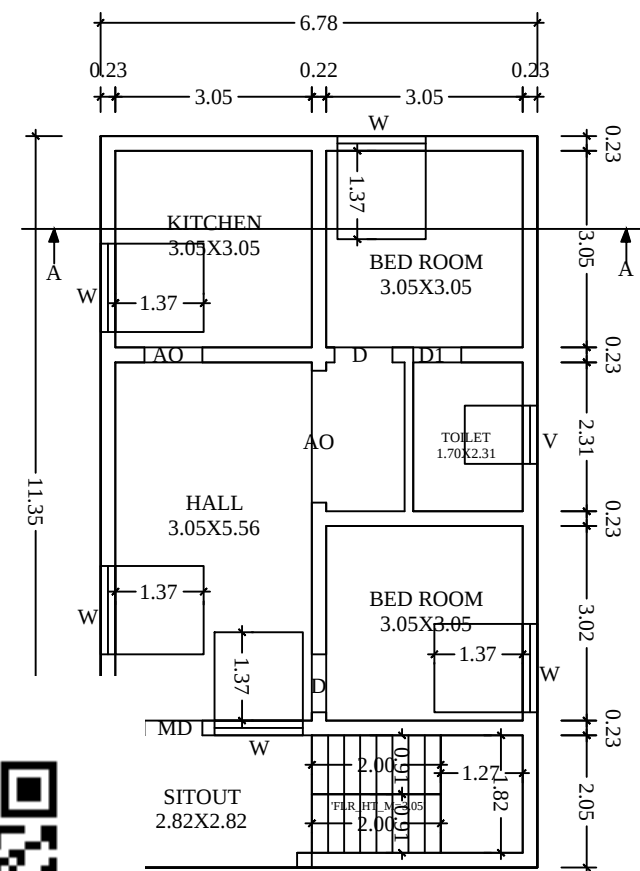
PLAN FOR GROUND FLOOR
