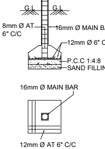
Column Footing Details: Column size - 9" x 12"
