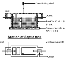
SEPTIC TANK DETAIL
