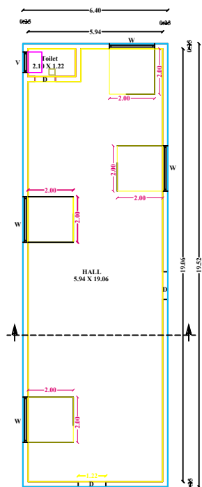
PROPOSED GROUND FLOOR
