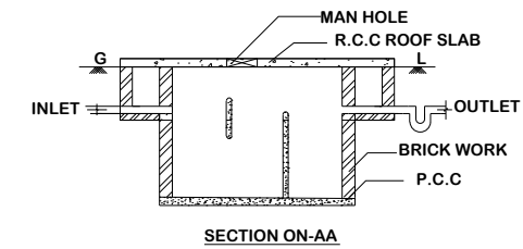
SECTION ON-AA
