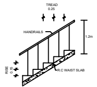
STAIRCASE DETAILS
