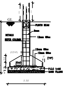
FOUNDATION DETAILS
