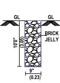
PERCULATION PIT
