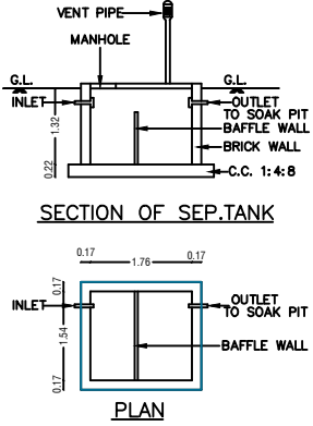
SEPTIC TANK
