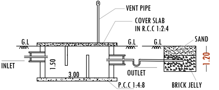
SECTION-AB
