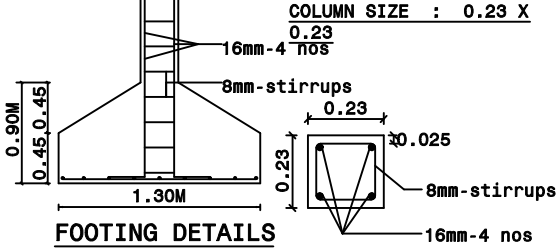
DETAILS OF COLUMNS
