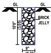
PERCULATION PIT
