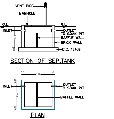
SEPTIC TANK
