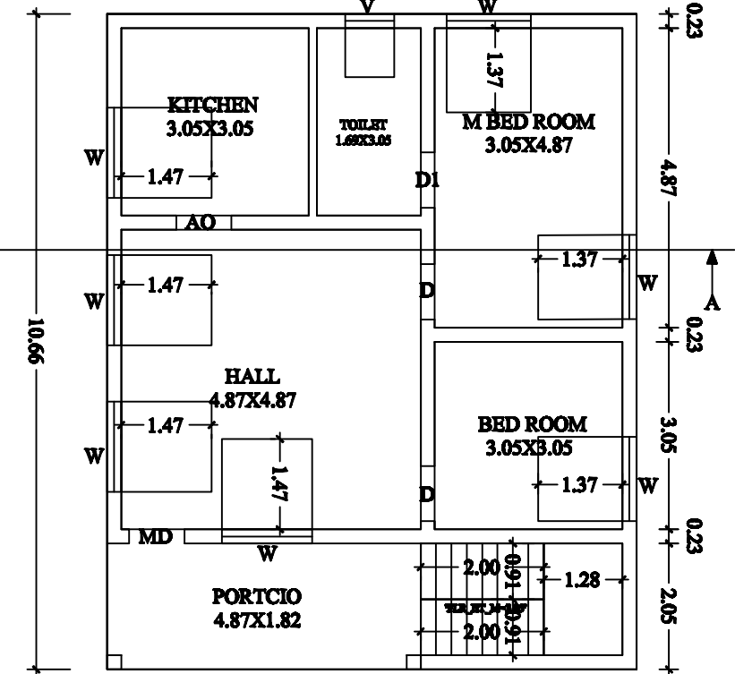
PLAN FOR FIRST FLOOR
