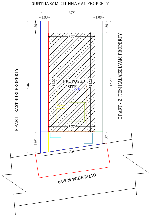
SITE PLAN
