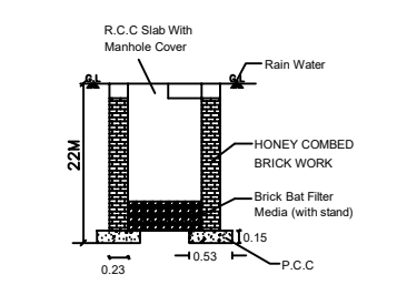
DETAILS OF RAIN WATER COLLECTION PIT RECHARGE WELL METHOD
