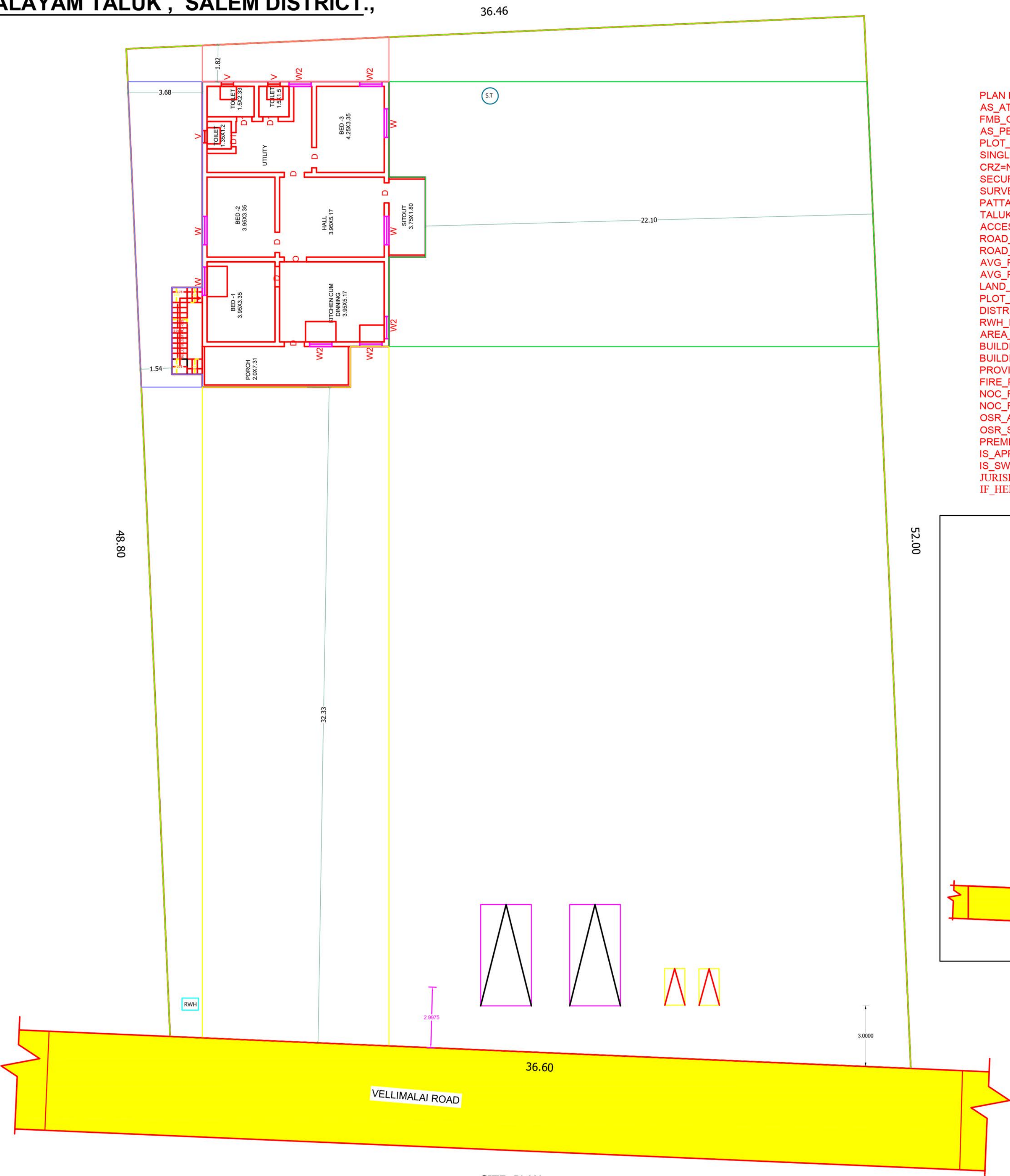
SITE PLAN
