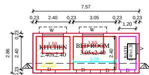
GROUND FLOOR PLAN ( SCALE 1:100)
