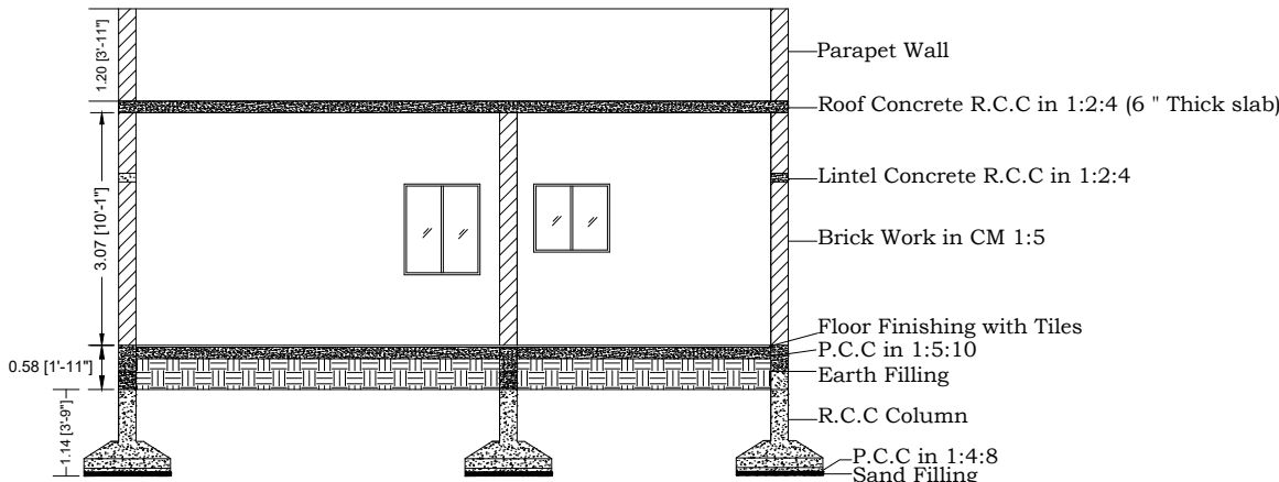
SECTION X-X
