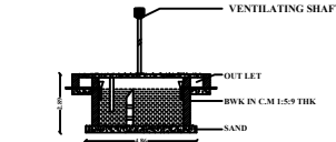
SECTION OF THE SEPTIC TANK
