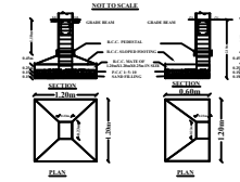
COLUMN FOOTING DETAILS
