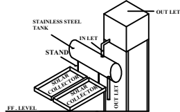
SOLAR HEATING WATER SYSTEM
