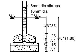
COLUMN FOUNDATION DETAIL
