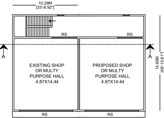
EXISTING & PROPOSED FIRST FLOOR PLAN
