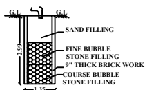
SECTION ON RAIN WATER COLLECTION TANK
