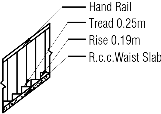
STAIR DETAILS
