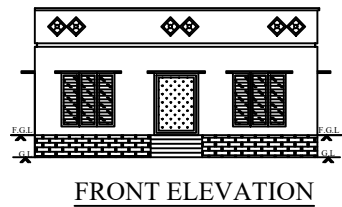
FRONT ELEVATION
