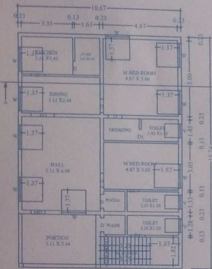
PLAN FOR GROUND FLOOR
