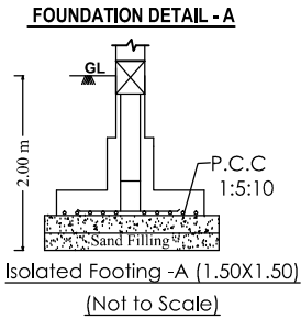
FOUNDATION DETAIL - A
