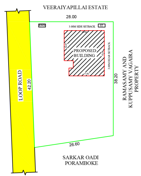
SITE PLAN (SCALE 1:400) (as per FMB)
