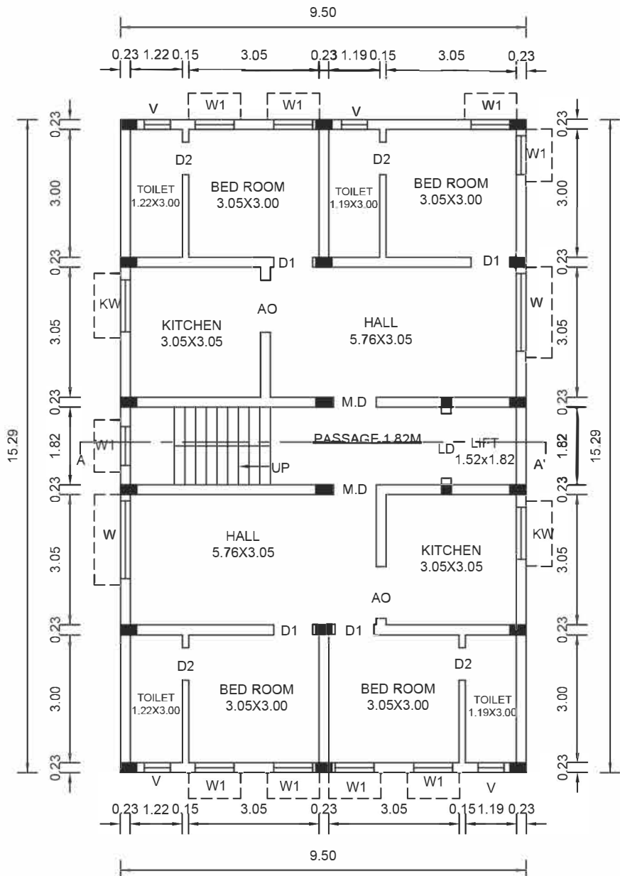
TYPICAL FIRST, SECOND, THIRD FLOOR
