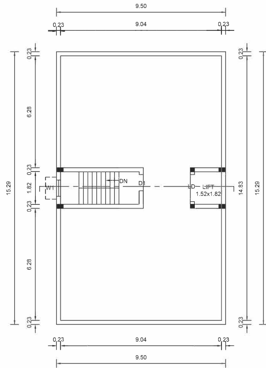
TERRACE FLOOR
