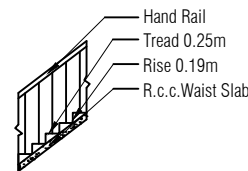
STAIR DETAILS
