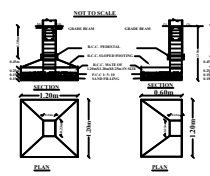
COLUMN FOOTING DETAILS
