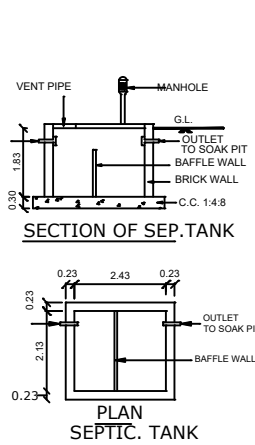
SEPTIC TANK:-
