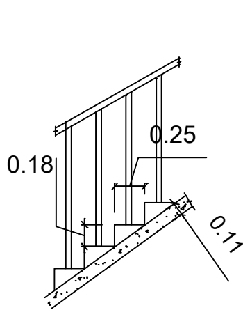
STAIRCASE DETAILS:-
