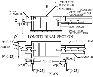
SEPTIC TANK:-
